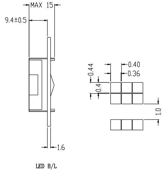
LED B/L
