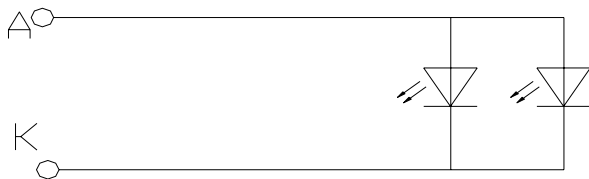
LED Sidelight circuit (color: White)
